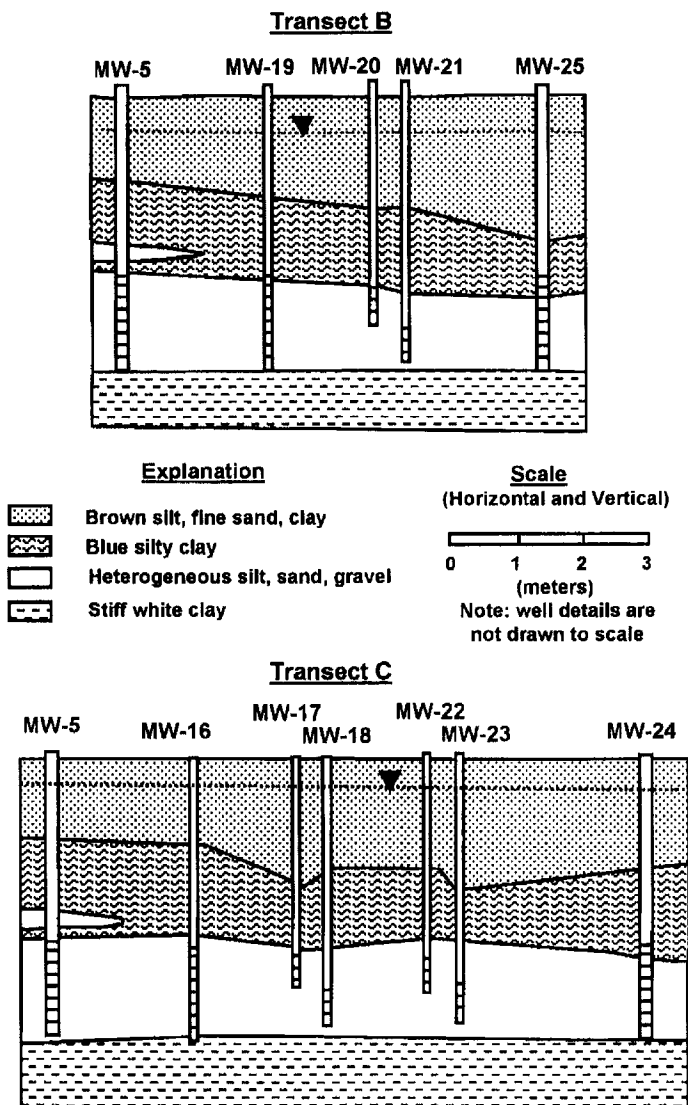
Figure 3. Transect cross sections.
